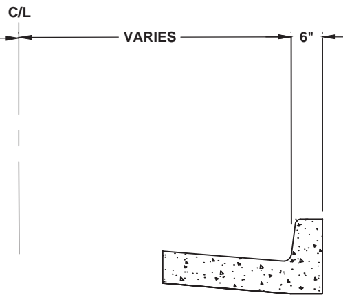
SECTION B-B STANDARD TYPE CURB & GUTTER THROUGH CATCH BASIN
