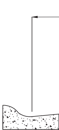
SECTION A-A ROLLED TYPE CURB & GUTTER
