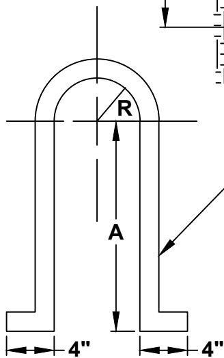
STRAP DETAIL
