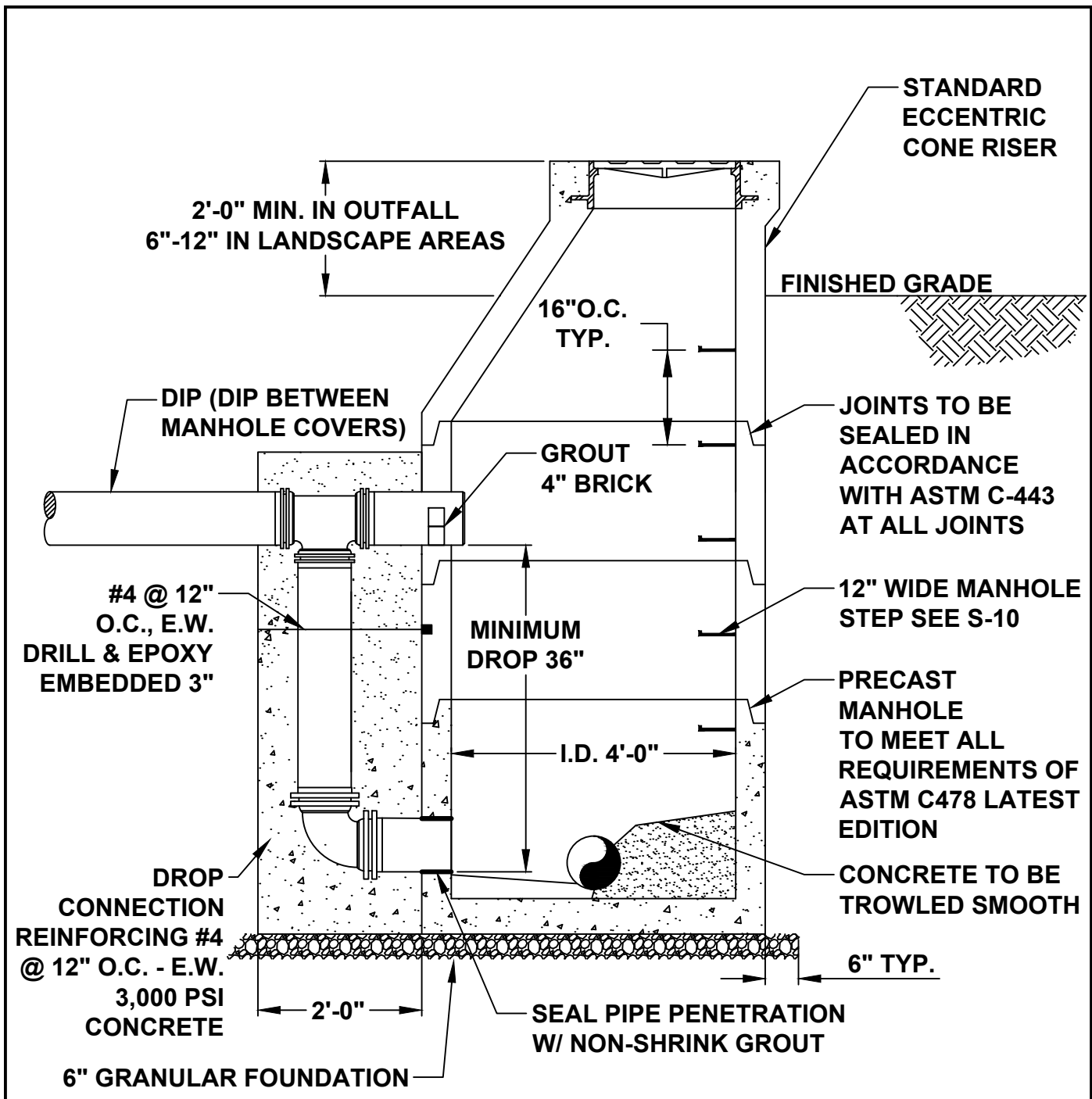
TYPICAL SECTION
