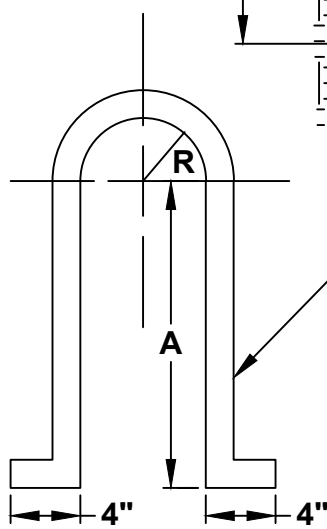
STRAP DETAIL
