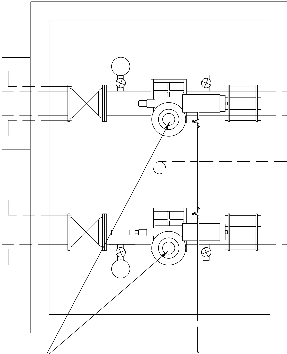
ECCENTRIC PLUG CHECK VALVE WITH HYDRAULIC CYLINDER OPERATOR BY DEZURICK
