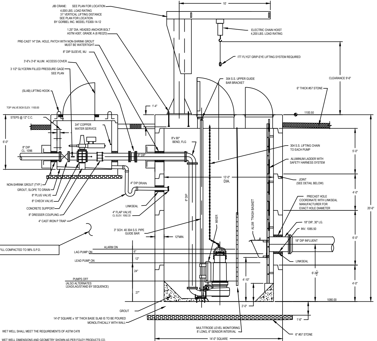
SECTION F-F
