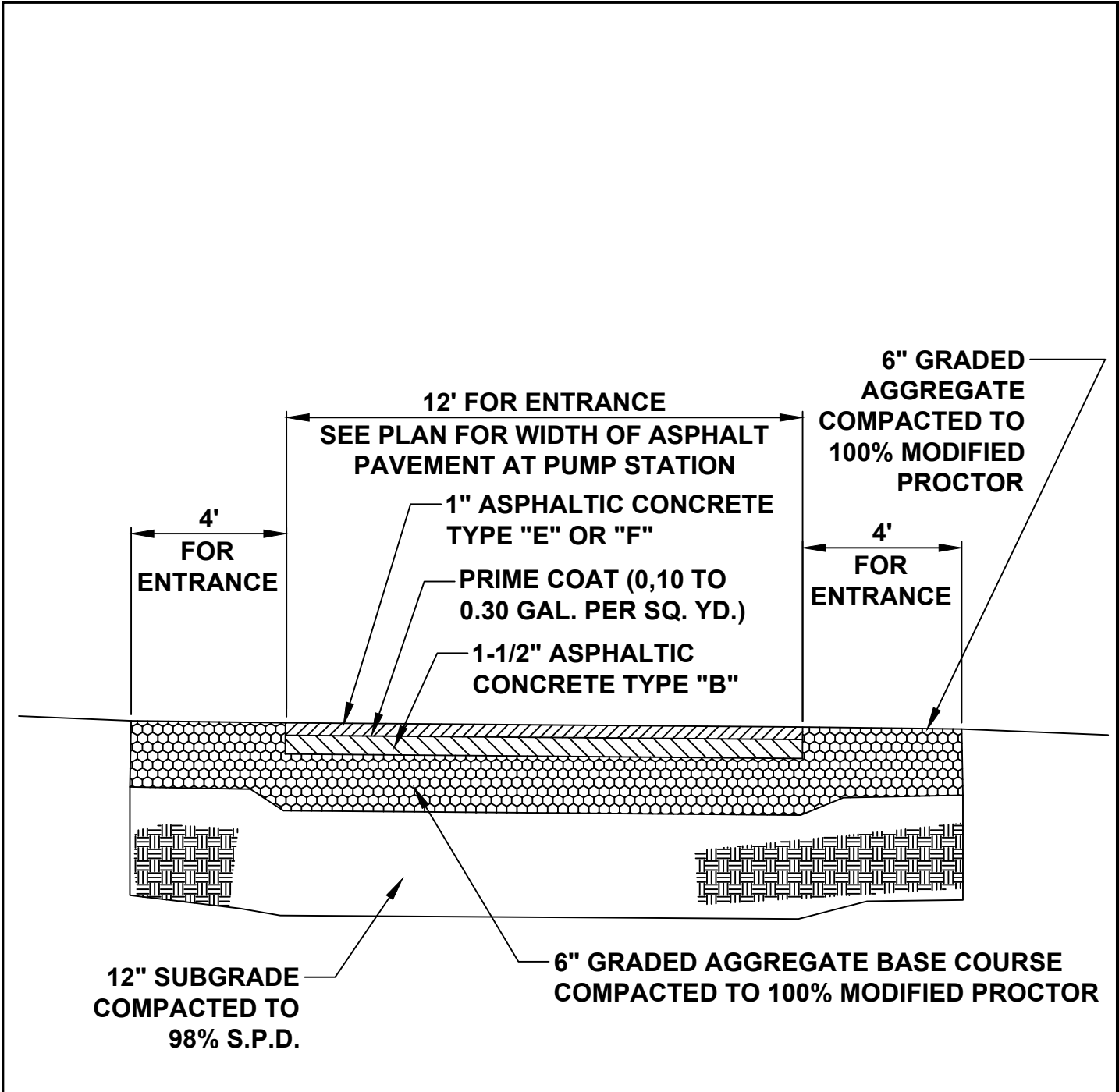
ASPHALT PAVING DETAIL
