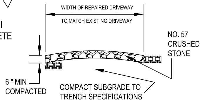
GRAVEL "A" - "A"
