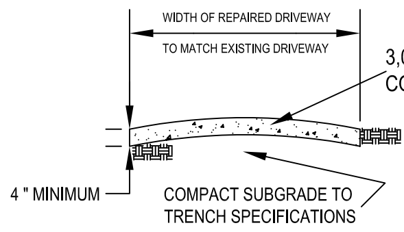
CONCRETE "A" - "A"
