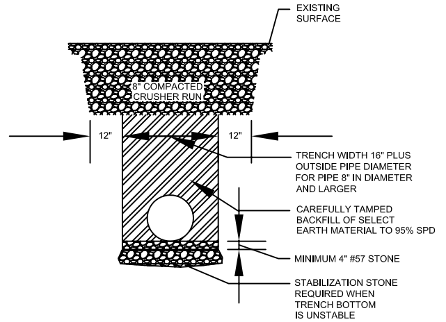
TYPE "B" CUT REPAIR DETAIL DIRT OR GRAVEL ROADS N.T.S.
