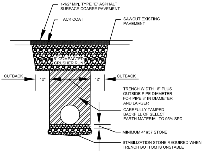
TYPE "A" CUT REPAIR DETAIL COUNTY ASPHALT ROADS N.T.S.
