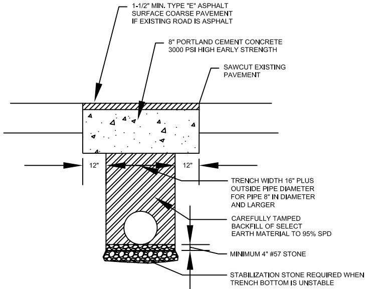
TYPE "C" CUT REPAIR DETAIL CONCRETE ROADS AND DOT ASPHALT ROADS N.T.S.
