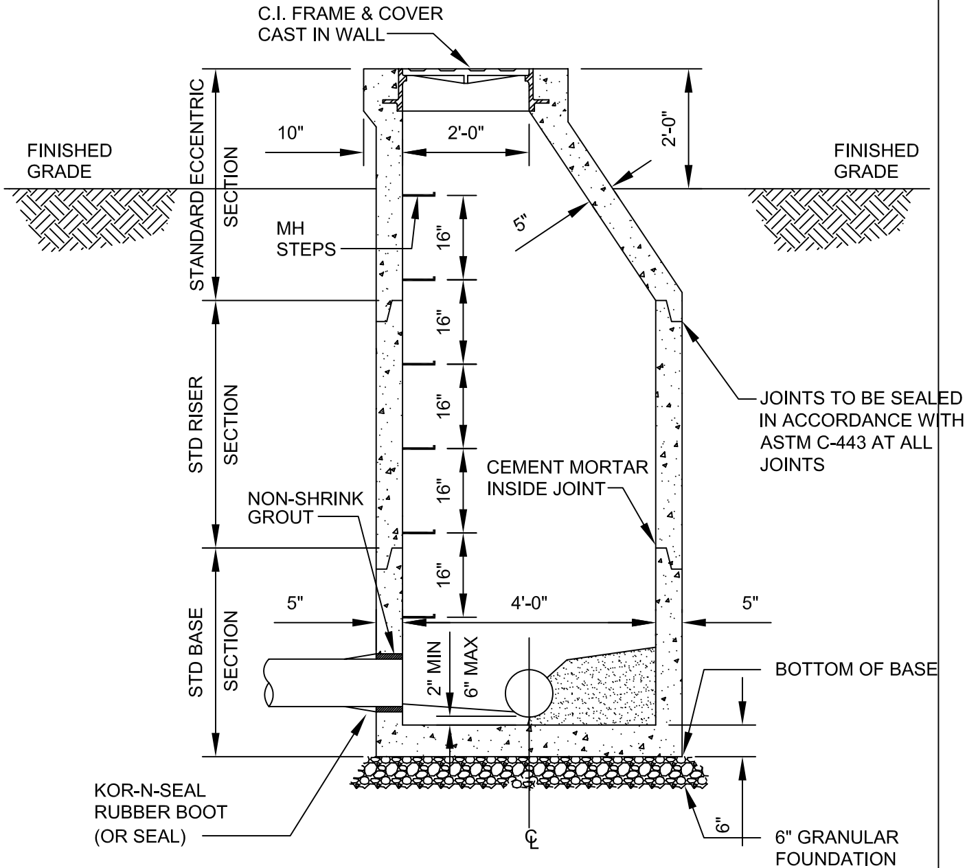
TYPICAL SECTION
