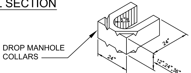
COLLAR DETAILS
