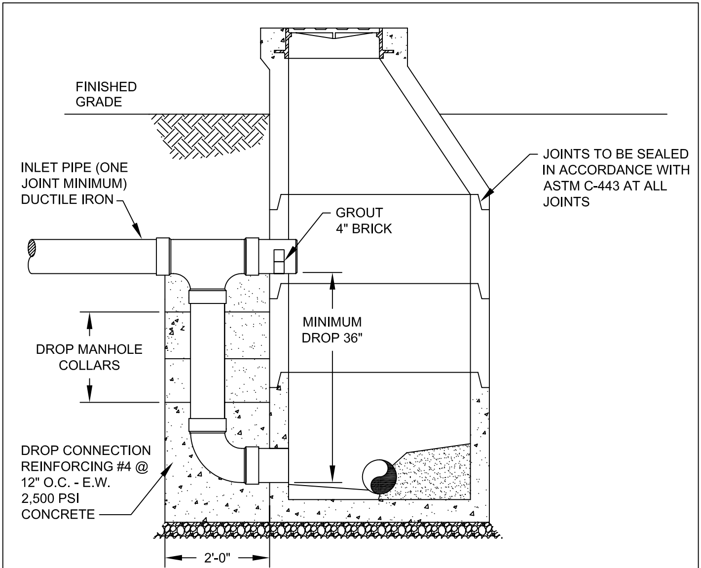
TYPICAL SECTION
