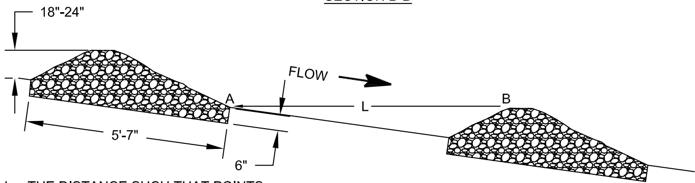
SECTION B-B
