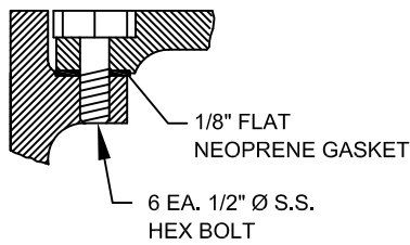
BOLT-DOWN DETAIL
