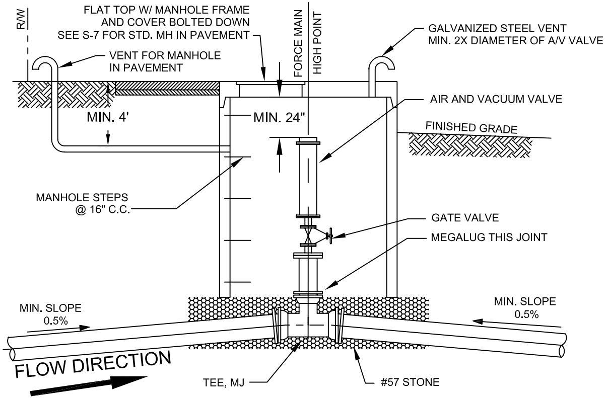
SECTION B-B
